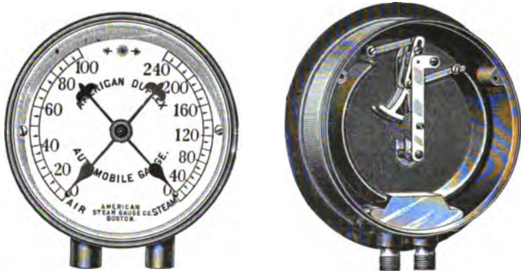
Figs. 141-141a. —Dial and Interior View of the "American" Duplex Combined Steam and Air Pressure Gauge for Use on Steam Carriages. The dial has two hands; one of them attached to a sleeve which works over the spindle carrying the other, in the same manner as the two hands of a clock are hung. As may be readily understood, the two hands work in opposite directions, one clockwise, the other counter-clockwise, from zero to maximum on their respective scales. The sectional view shows the mechanism by which this result is accomplished: two separate inlets, for steam and air, respectively; two distinct flattened and curved steel tubes, each attached at its end by a link to a lever and toothed sector working on the toothed pinion concentric with the pivot of one of the hands. The two flattened tubes, of course, have different tensile ratios, causing them to tend to straighten at different pressures. Hence the steam hand records a maximum pressure of 240 pounds, while the air hand records a maximum pressure of 100 pounds. Duplex gauges of precisely the same construction are used on the air-brake systems of many railroad locomotives—one hand recording the pressure in the air reservoir, the other in the train pipe. The duplex spring used in this make of gauge is so well constructed and so sensitive that it enables the manufacture of the smallest size of gauges on the market. A duplex gauge of this description is shown in place on a steam carriage in Fig. 247.
